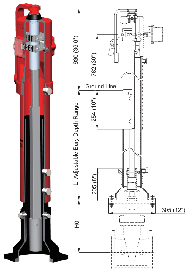
FIG. F0800-IP (Size 4" to 14")
